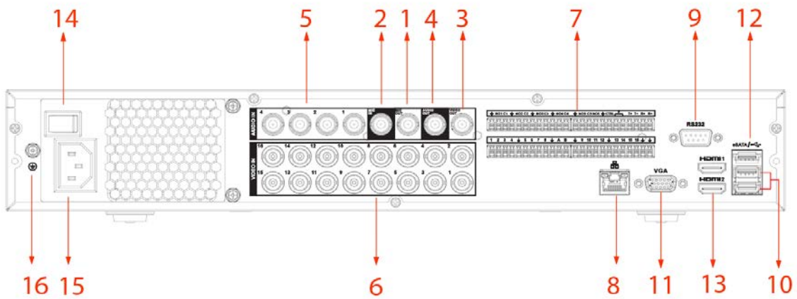
Figure 3-20 Rear panel (3)
