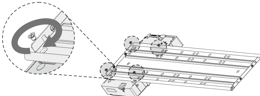
Figure 2-19 Fix HDD
